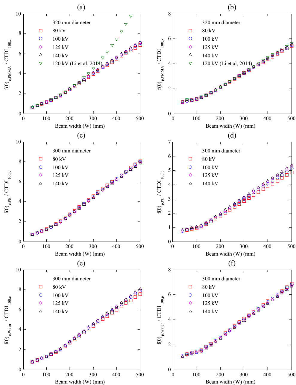
Figure 6. f(0)_{x,m} values calculated within 600 mm long body phantoms of different compositions using beams of width W = 40\text{--}500 mm and normalized with respect to \text{CTDI}_{100,x} measured at the same position within a 150 mm long PMMA body phantom (centre and periphery) and with the same beam widths. (a)–(b) PMMA, (c)–(d) PE, and (e)–(f) water body phantoms (table 1). PMMA results are compared with values reported in Li et al (2014) at 120 kV.
