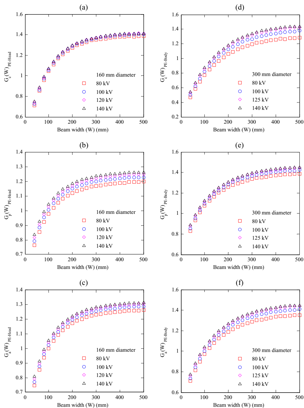
Figure 3. G_c(W) , G_p(W) , and G_a(W) functions for f(0)_{x,\text{PE}} values calculated within 600 mm long PE phantoms and normalized with respect to \text{CTDI}_{w,40} values calculated within 150 mm long PMMA phantoms as in equation (5) using beams of width W = 40\text{--}500 mm. (a)–(c) for the head phantoms and (d)–(f) for the body phantoms (table 1).
